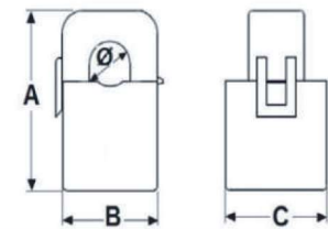
Dimensions(mm/inch)
